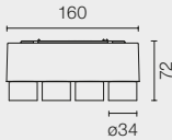
POWER LED 10W
