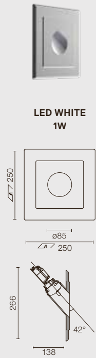
ROUND LIGHT SMALL
