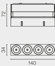
POWER LED 10,8W
