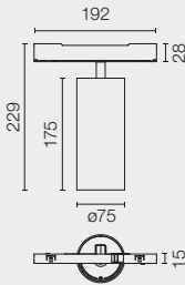
LED ARRAY 35,3W
