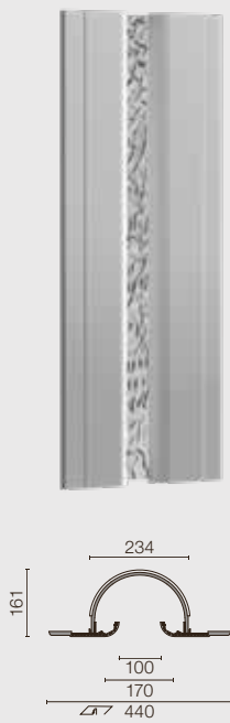
SOFTPROFILE DECO STARCK LARGE
