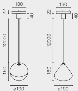
POWER LED 16W
