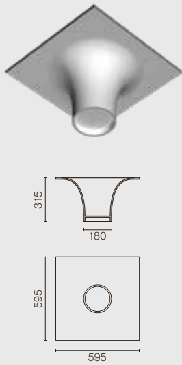
USO BOOB 600 FOR MODULAR CEILING
