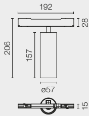
LED ARRAY 23,5W
