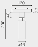
POWER LED 12,5W/14W DALI
