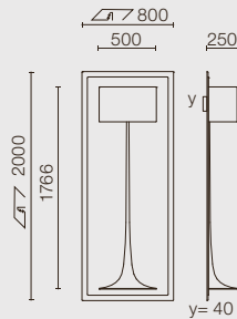
TC-L 24W (diffuser) LED WHITE 1,4W
