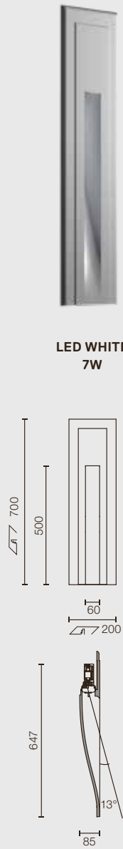
VERTICAL LIGHT LARGE
