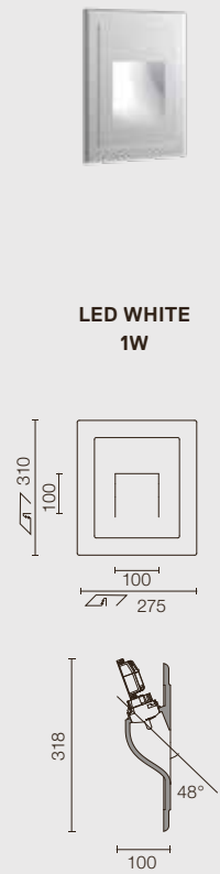
SQUARE LIGHT SMALL
