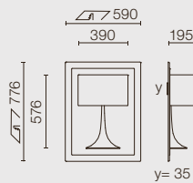
LED WHITE 35W
