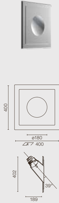
ROUND LIGHT MEDIUM
