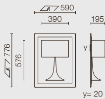
QT-DE-12 max 120W
