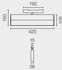
TOP LED 25,5W
