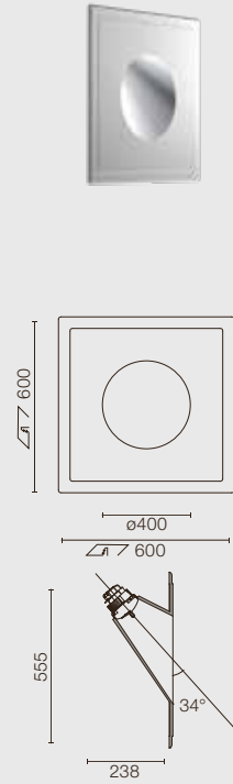
ROUND LIGHT LARGE
