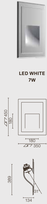
SQUARE LIGHT LARGE
